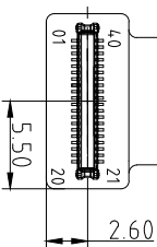
BOTTOM VIEW
